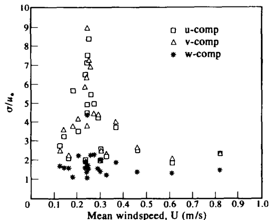
Fig. 1. Scatter diagram showing the variation of standard deviation of wind components normalized by the friction velocity with horizontal mean wind speed for U < 1 \text{ m s}^{-1} .
