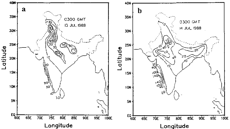
Figure 3 Accumulated rainfall ( \text{mm d}^{-1} ) ending at 0300 UTC. (a) 13 July 1988, (b) 14 July 1988.
