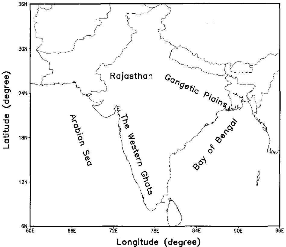
Figure 1 Geography of India and its surrounding regions.
