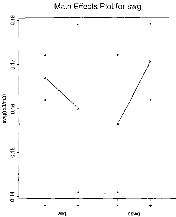
Figure 10. Main-effect plot for surface soil moisture (resolution V experiment).
