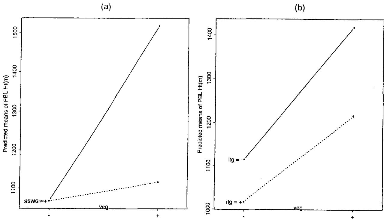
Figure 6. Two-factor interaction plots for (a) deep soil moisture ( \text{m}^3/\text{m}^3 ) and vegetal cover interaction, and (b) initial ground temperature (K) and vegetal cover interaction, for PBL height prediction. (Confidence level is \sim 90\% based on pseudo standard error.)
