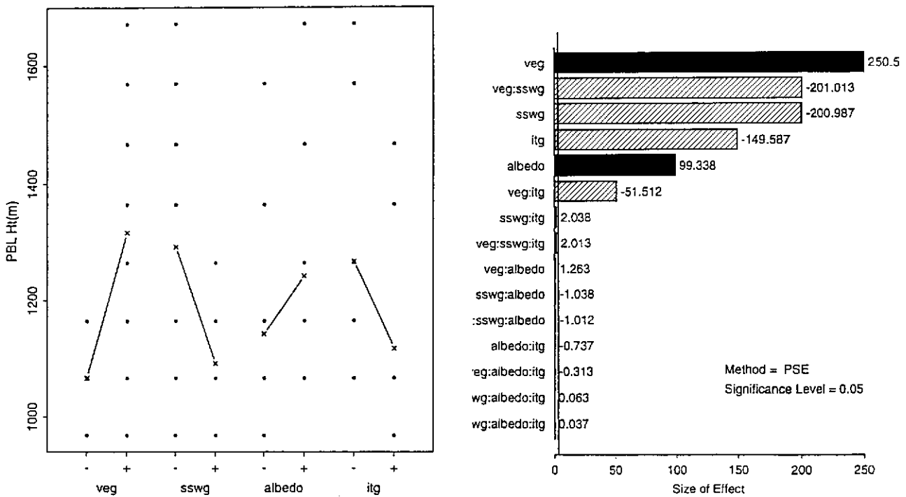
Figure 5. Main-effect and Pareto plots for PBL height (resolution V experiment).
