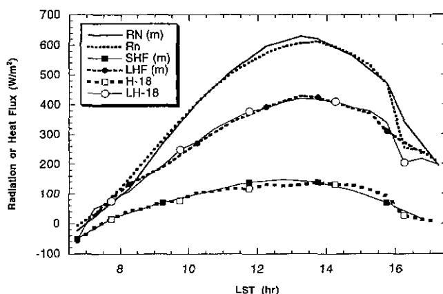
Figure 1. Comparison between FIFE-observed and model-predicted surface parameters. R_n and RN(m) are observed and modeled net radiation, H-18 and SHF (m) are the observed and modeled sensible heat fluxes, LH-18 and LHF (m) are the observed and modeled latent heat fluxes for the FIFE site 18.
