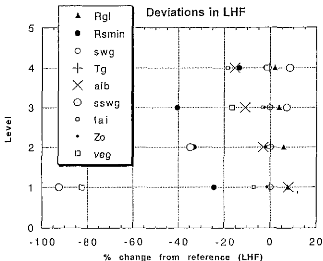
Figure 4. An OAT outcome for LHF ( W/m^2 ) predictions from the model. "Level" indicates the parameter quartile settings shown in table 2.
